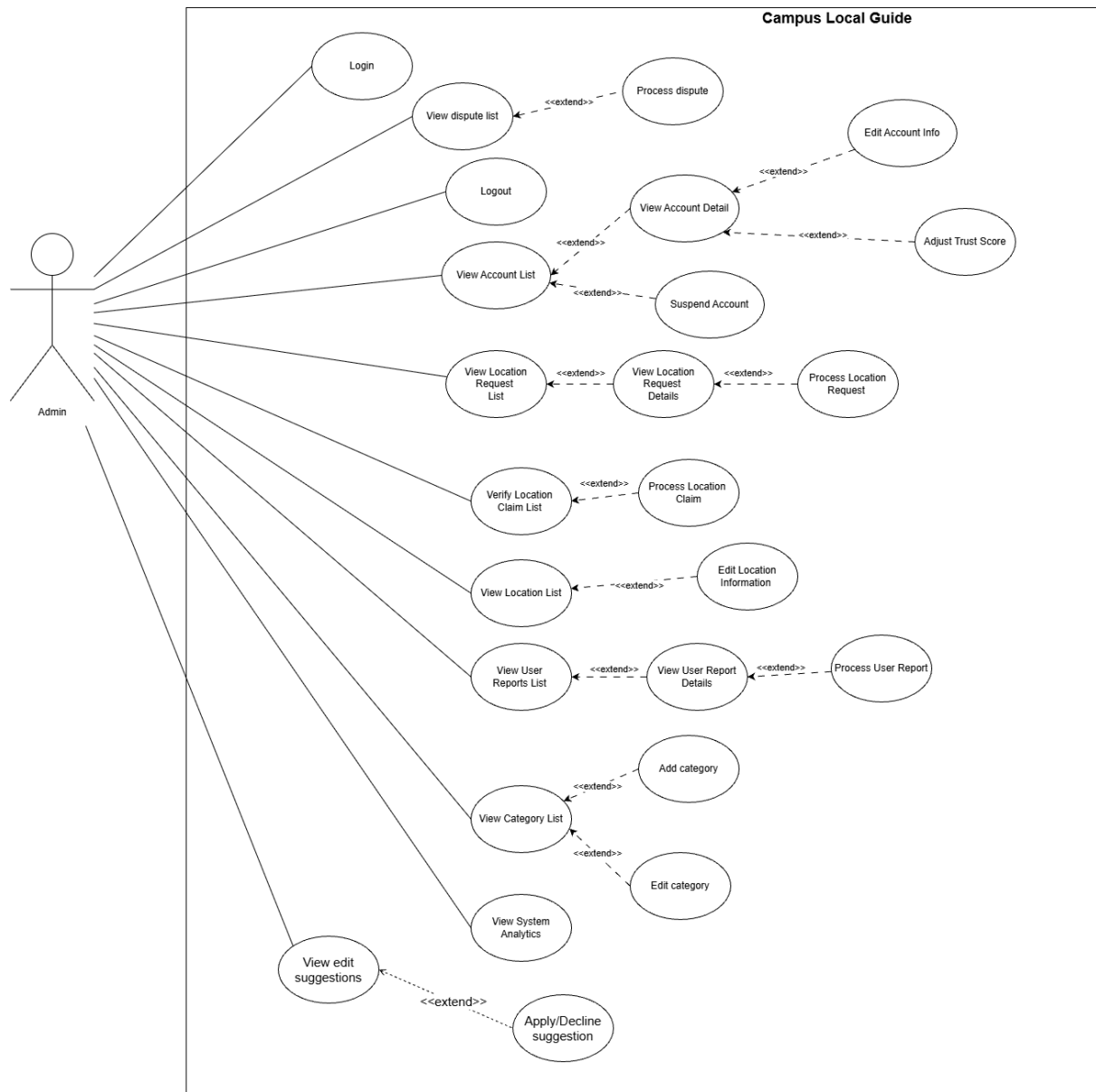
Admin Use Case Diagram
