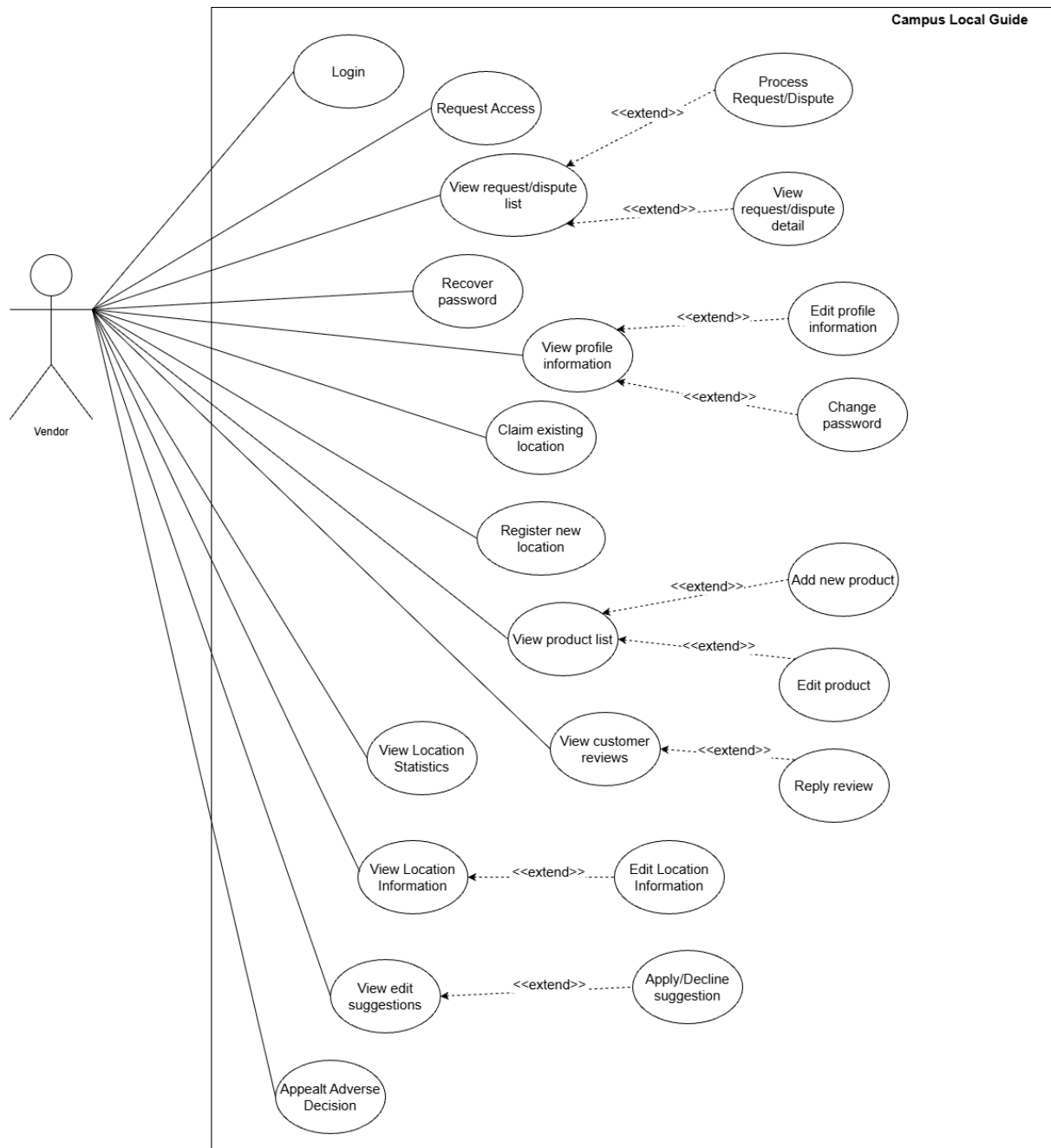
Vendor Use Case Diagram
